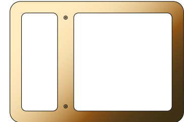
riv 206 C w 449 x h 314 x d 15 (93x254)+(254x254)mm w 17,68 x h 12,36 x d 0,59 (3,66x10)+(10x10)"
